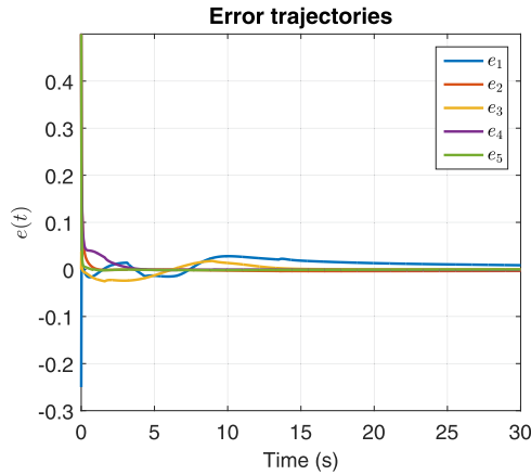
Fig. 3. Tracking error trajectories for the agents for the one-dimensional example.
