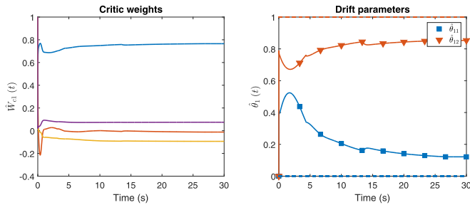
Fig. 5. Value function weights and drift dynamics parameters estimates for Agent 1 for the one-dimensional example. The dotted lines in the drift parameter plot are the ideal values of the drift parameters.
