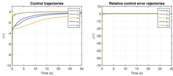
Fig. 4. Trajectories of the control input and the relative control error for all agents for the one-dimensional example.
